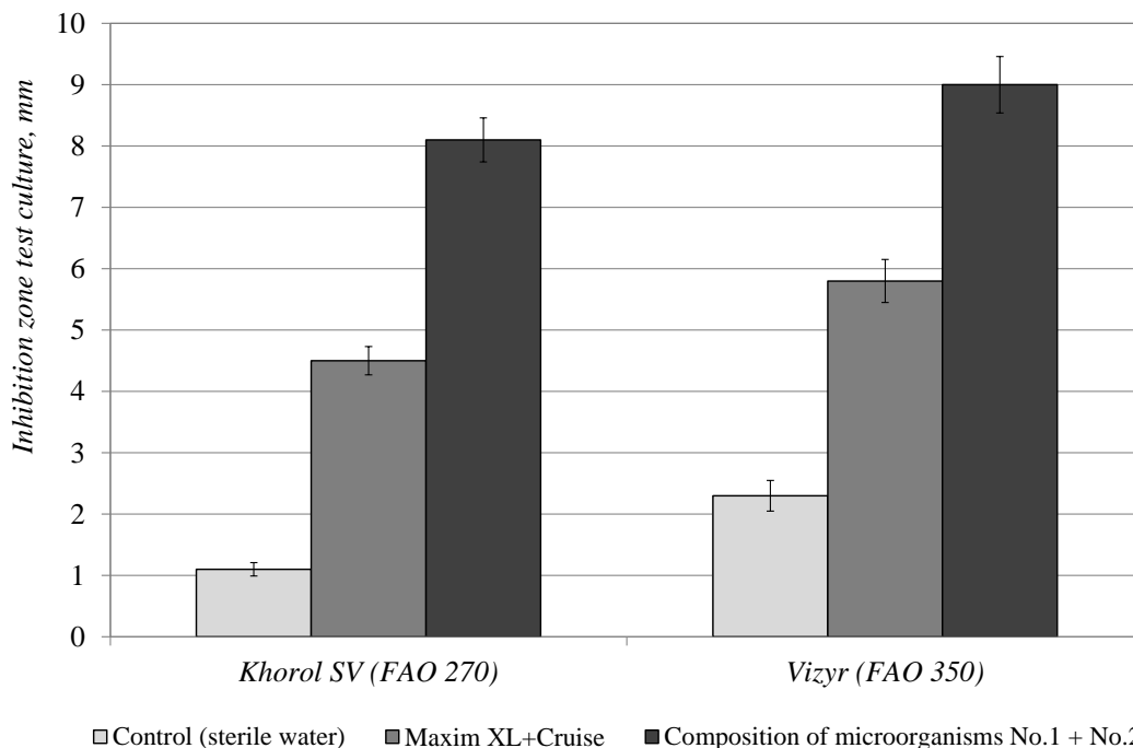
Figure 1. Antifungal activity of the soil of the root zone of corn when using a complex of compositions of microorganisms No.1+No.2 and chemical preparations
